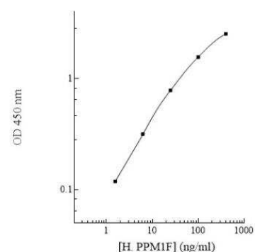
Human PPM1F Standard Curve
