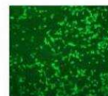
CHIKV-infected
